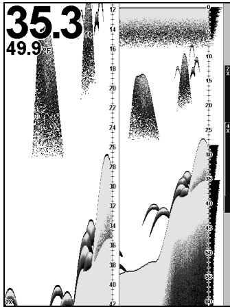
Sonar page in Split Zoom Sonar Chart display mode.
